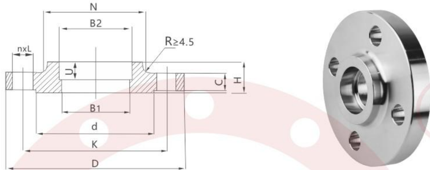
承插焊钢制管法兰 HG/T20619-2009(SW) SOCKET WELDED STEEL PIPE FLANGE
